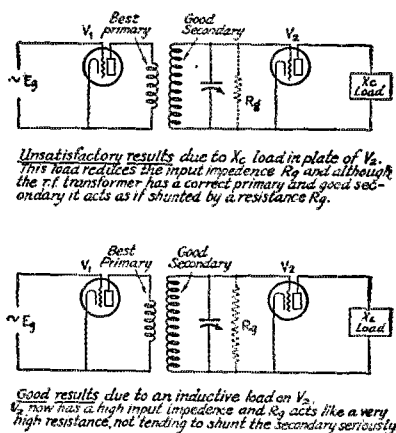
FIG. 3—THE EFFECT OF PLATE LOAD
