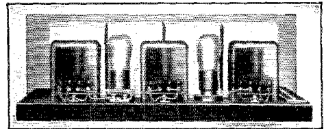
REAR VIEW OF WIRED SET WITH SHIELDS IN PLACE
