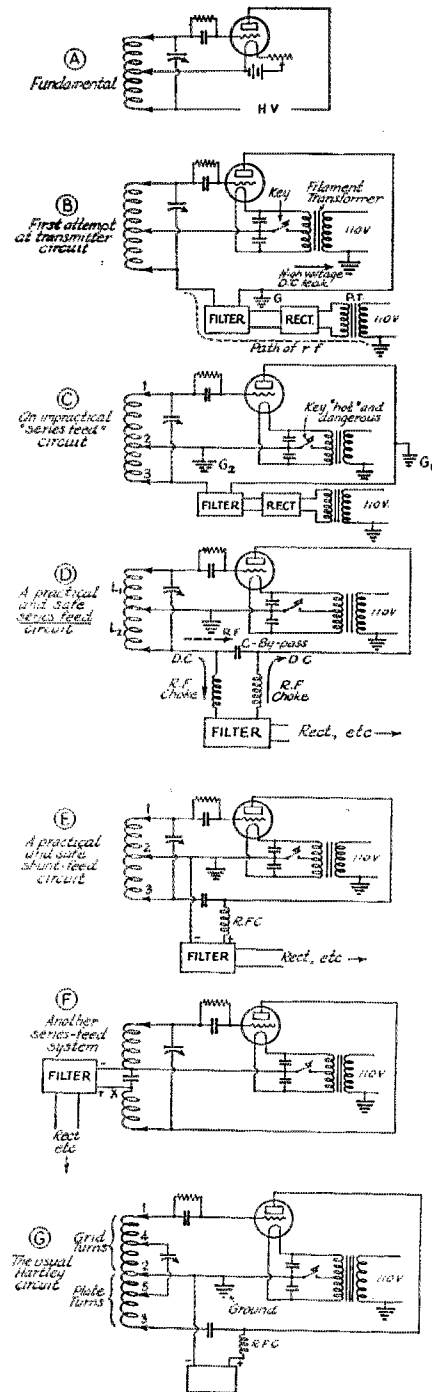
FIG 3 — DEVELOPING PRACTICAL SENDING CIRCUITS
