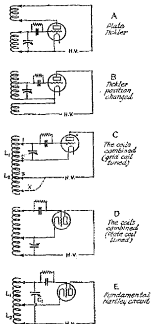
FIG. 2 — DEVELOPING THE HARTLEY CIRCUIT FROM THE PLATE-TICKLER-CIRCUIT
